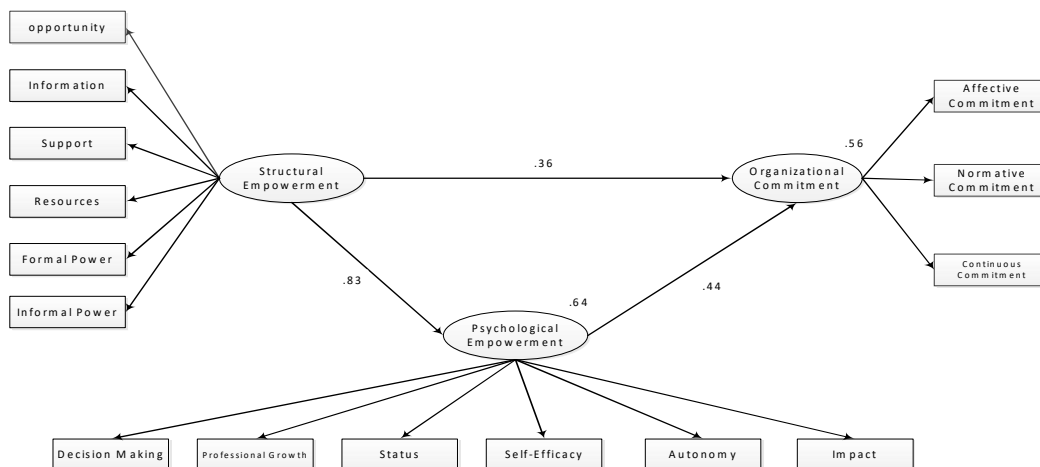
Figure 2 Hypothesized model with path coefficients
