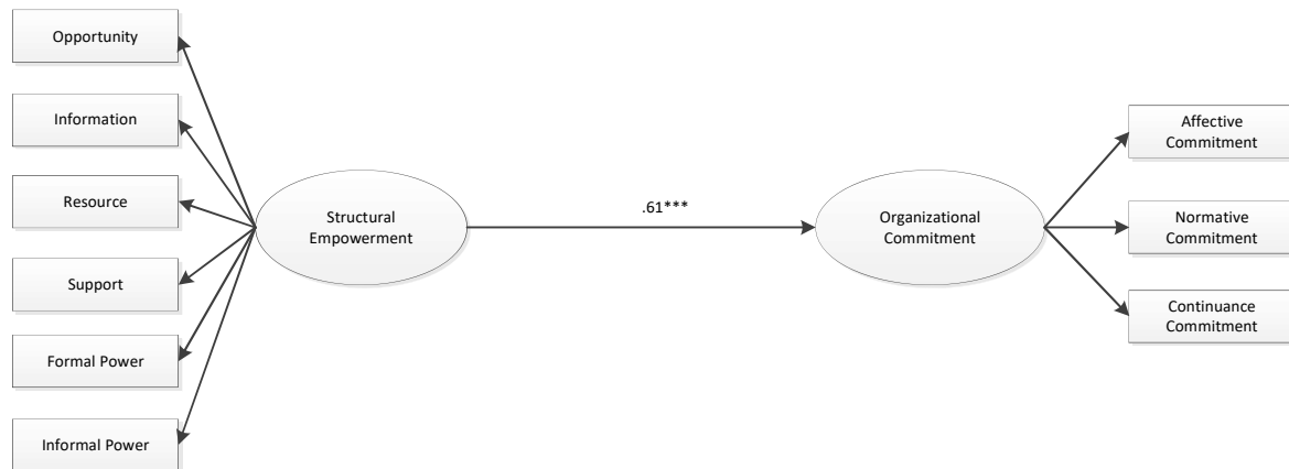
Figure 1 Direct effect of path coefficient
