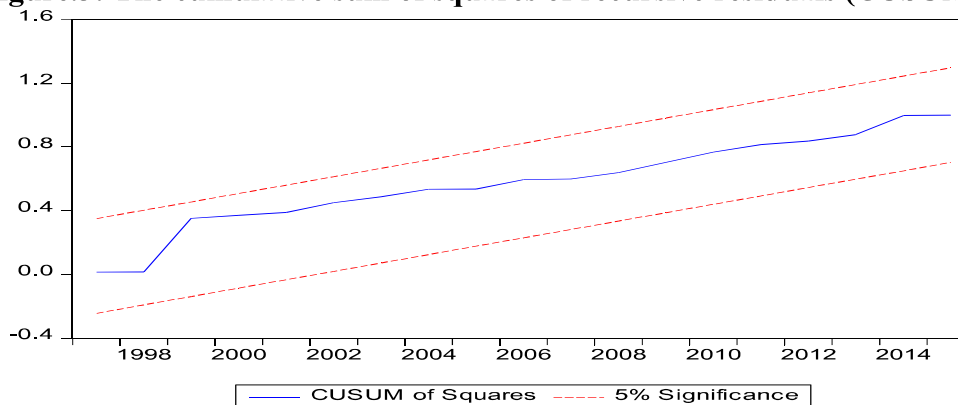
Figure.3: The cumulative sum of squares of recursive residuals (CUSUMQ)
