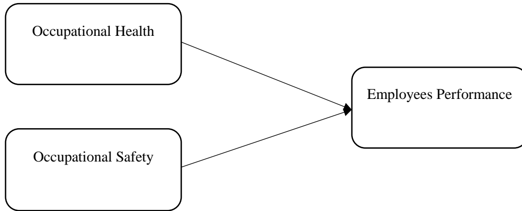
Figure 1 Theoretical framework
